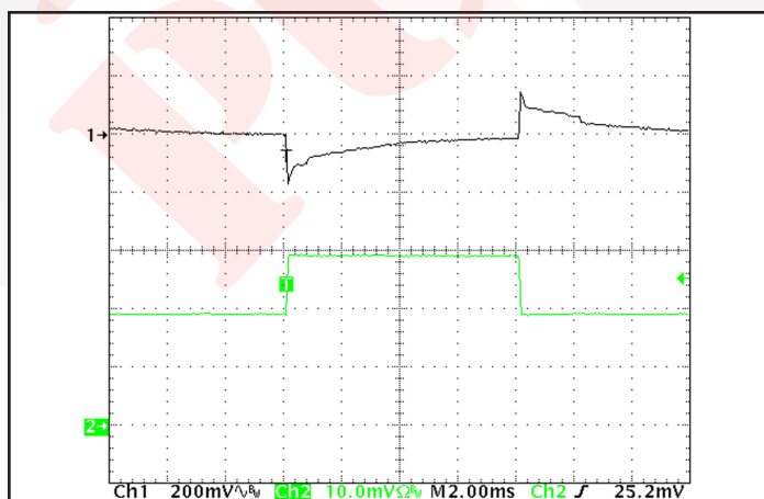
Figure 11: Output voltage response to step-change in load current (50%-75%-50% of Iout(max); dI/dt = 0.1 \text{ A}/\mu\text{s} ). Load cap: 1 μF ceramic and 15 μF tantalum capacitors. Ch 1: Vout (200mV/div), Ch 2: Iout (10A/div).
