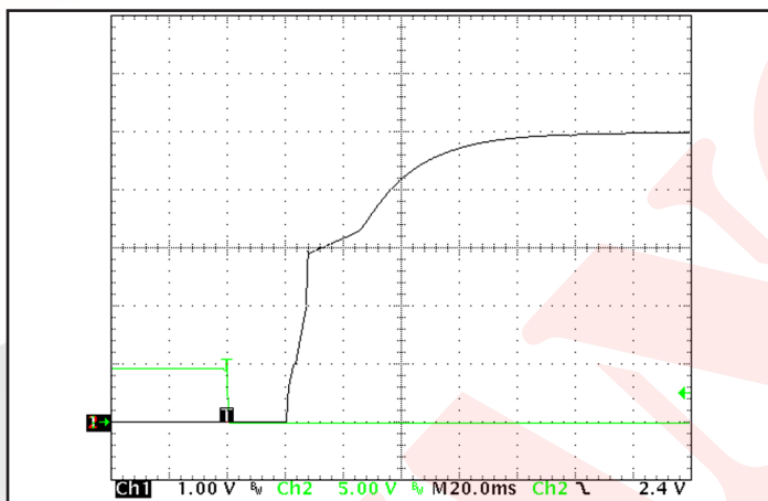
Figure 7: Typical startup waveform. Input voltage pre-applied, CH1: Vout (1V/div), CH2: ON/OFF (5V/div), Horizontal scale (20ms/div).
