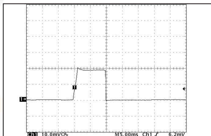
Figure 18: Load current (50A/div) as a function of time (5ms/div) when the converter attempts to turn on into a 10 m \Omega short circuit.
