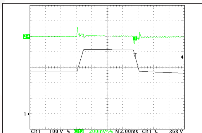
Figure 12: Output voltage response to step-change in input voltage (250V/ms). Load cap: 1 μF ceramic and 15 μF tantalum capacitors. Ch 1: Vin (100V/div), Ch 2: Vout (200mV/div).
