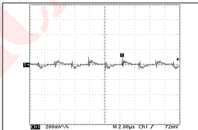
Figure 10: Output voltage ripple, Vout, at nominal input voltage and rated load current (200 mV/div). Load capacitance: 1μF ceramic capacitor and 15μF tantalum capacitor. Bandwidth: 10 MHz. See Figure 17.
