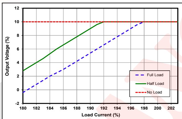
Figure 19: Maximum allowable trim at -55C over line.
